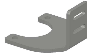
UPPER BRACKET (1:4)
