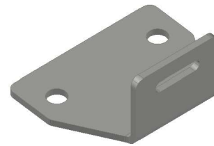
LOWER BRACKET (1:4)
