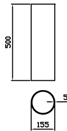
60242 Plasthylse for trestolp
