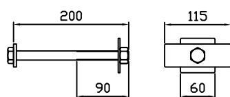
60602 Festesats for trestolp m/plasthylse M16x200
