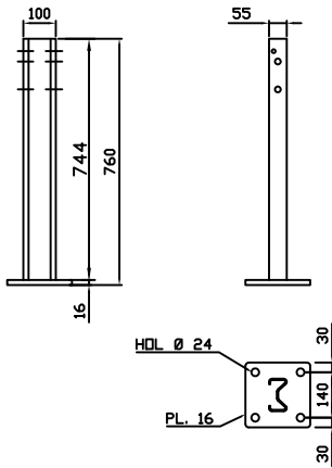
60230 Sigmastolp L=760 m/fotpl. 200x200x16
